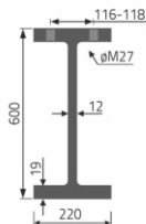
IPE 600
